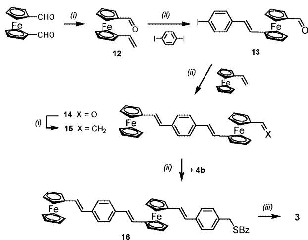
Scheme 3. Synthesis of compound 3 : (i) methyltriphenylphosphonium bromide, tert -butoxide, dioxane/water; (ii) \text{Pd}(\text{OAc})_2 , \text{P}(\text{Tol})_3 , tributylamine, dimethylacetamide; (iii) \text{NaBH}_4 , THF, MeOH, 0 °C.
