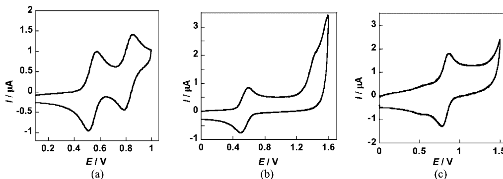
Figure 1. Cyclic voltammogram of (a) 14 ( 3.8 \times 10^{-4} M), (b) 16 ( 2.5 \times 10^{-4} M), (c) 17 ( 2.7 \times 10^{-4} M) in dichloromethane containing 0.1 M TBABF 4 at a scan rate of 0.2 \text{ Vs}^{-1} .
