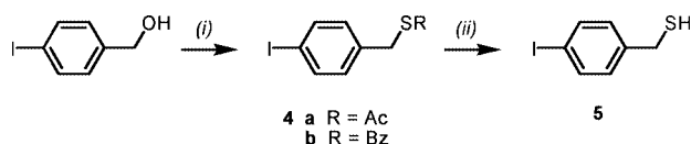
Scheme 1. Synthesis of the precursors 4a and 4b : (i) AcSH (for 4a ), BzSH (for 4b ), PPh 3 , DEAD, THF, 0 °C; (ii) LiAlH 4 , THF, 0 °C.
