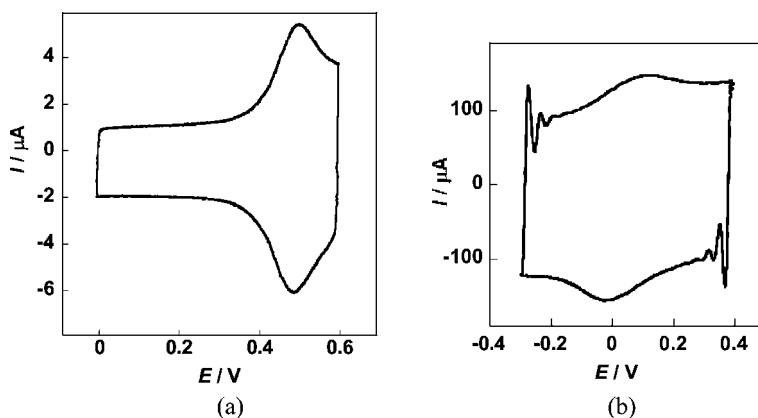
Figure 2. Cyclic voltammogram in 1 M perchloric acid of 3 coadsorbed (a) with pentanethiol onto a 111 gold single-crystal electrode, scan rate: 12 V s -1 ; (b) with diphenyl disulfide onto a gold ball ultramicroelectrode, scan rate: 220000 V s -1 .
