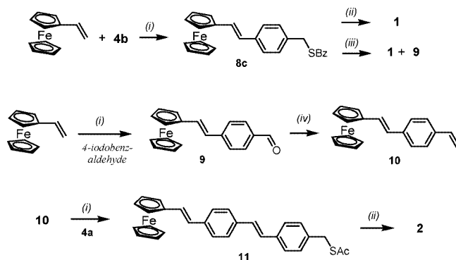
Scheme 2. Synthesis of compounds 1 and 2 : (i) Pd(OAc) 2 , P(Tol) 3 , tributylamine, dimethylacetamide; (ii) NaBH 4 , THF, MeOH, 0 °C; (iii) LiAlH 4 , THF, 0 °C.
